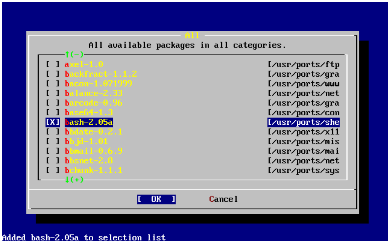
Added bash-2.05a to selection list
